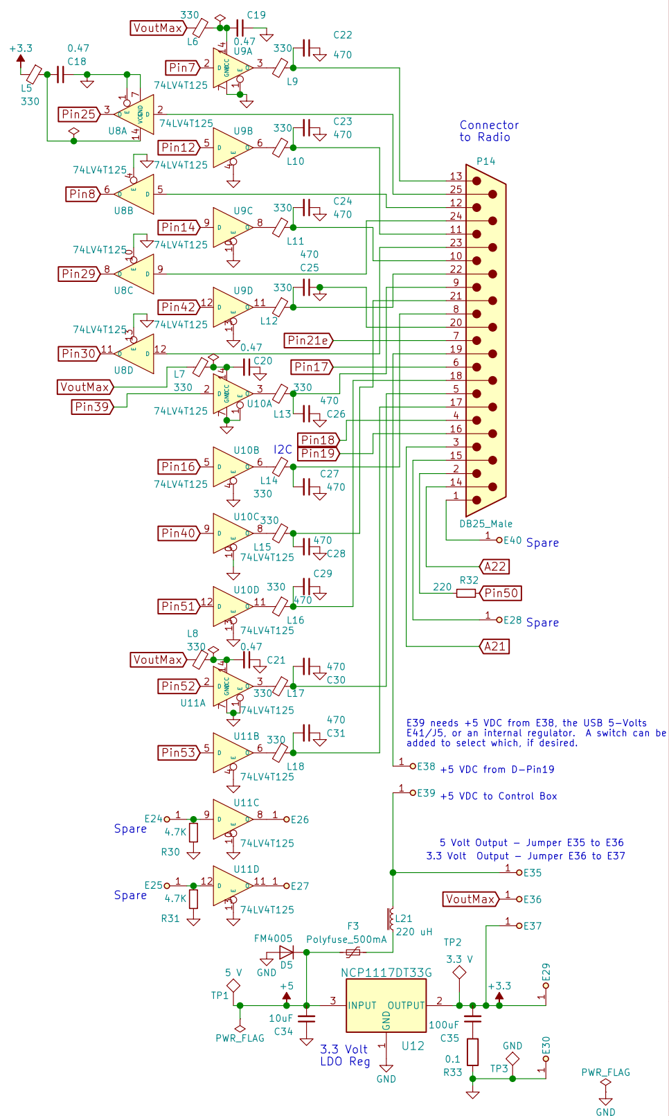
Schematic Diagram SDR Processor and Control W7PUA Version 0.4.1
